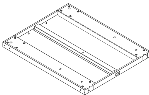
(#4-A2) Bottom Panel - Right x 1 PC
