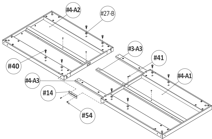
(#4-A) Bottom Panel
