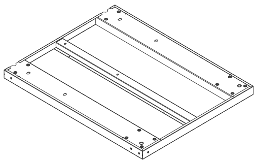
(#4-A1) Bottom Panel - Left x 1 PC
