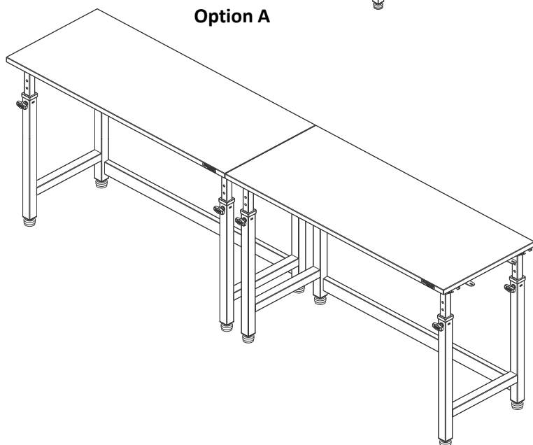
Option A. Connecting Side-by-Side
