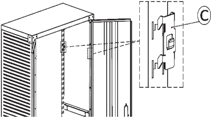
Right Side of Cabinet
