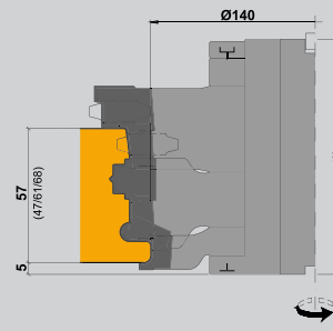
Top rail and stiles ID 955513 / 71100x
