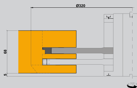
Top rail and stiles ID 955513 / 71100x
