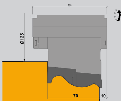
Optional horn 1 ID 955531 / 71100x
