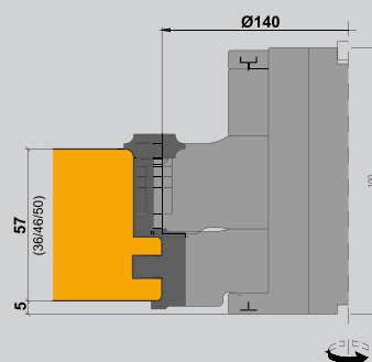
Frame inner profile ID 955525
