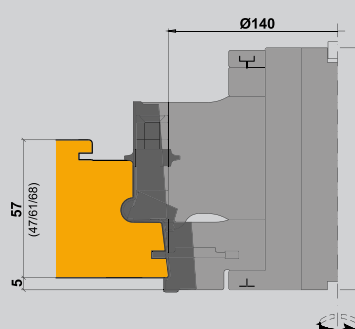
Optional horn 1 ID 955531 / 71100x
