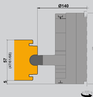
Rope groove ID 955527 / 71100x
