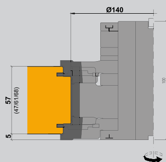
Outside bottom rail ID 955528 / 71100x
