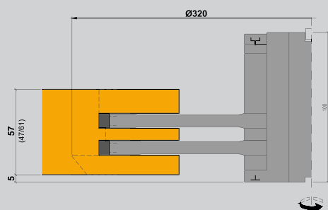
Inside sash profile ID 955512 / 71100x
