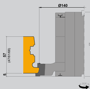
Outside sash egress profile ID 955515 / 71100x
