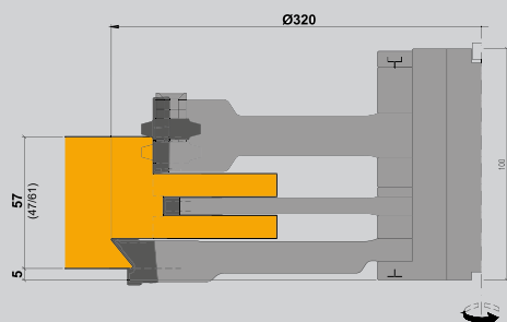
Sash slots ID 955510 / 71100x
