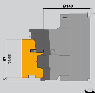
Optional bottom rail jointing
