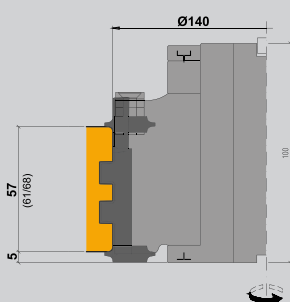
Open in door ID 955522 / 71100x
