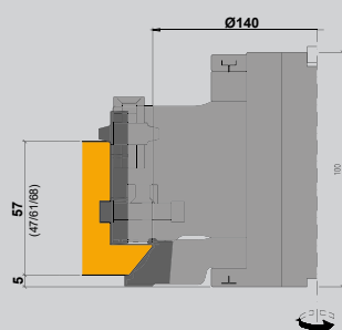
Outside sash bottom rail ID 955514 / 71100x
