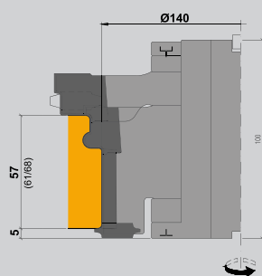
Open out door ID 955518 / 71100x
