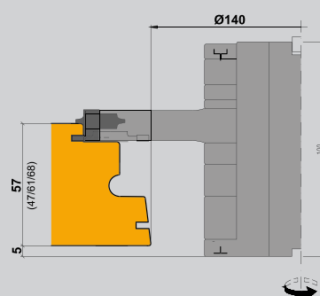
Frame inner profile ID 955525
